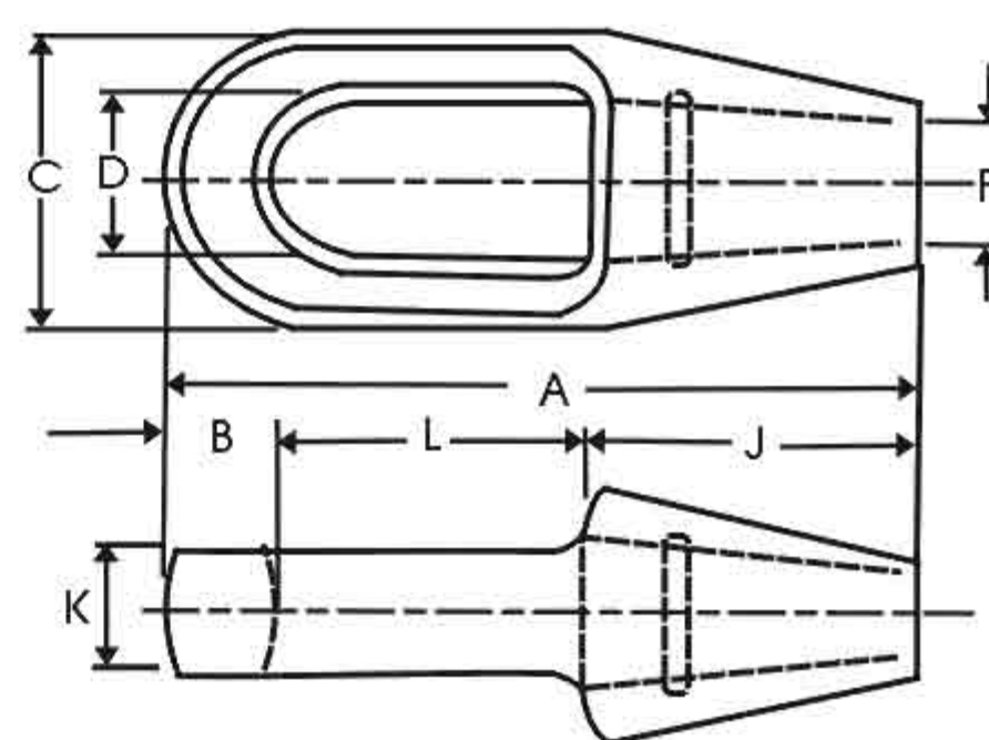
CLOSED SPELTER SOCKETS
